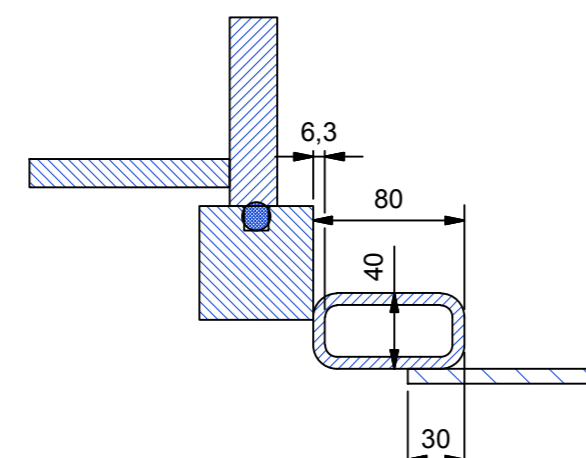
D-D Typical welding.
