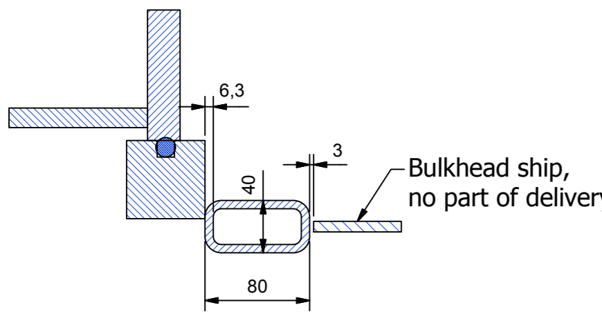
C-C Typical welding.
