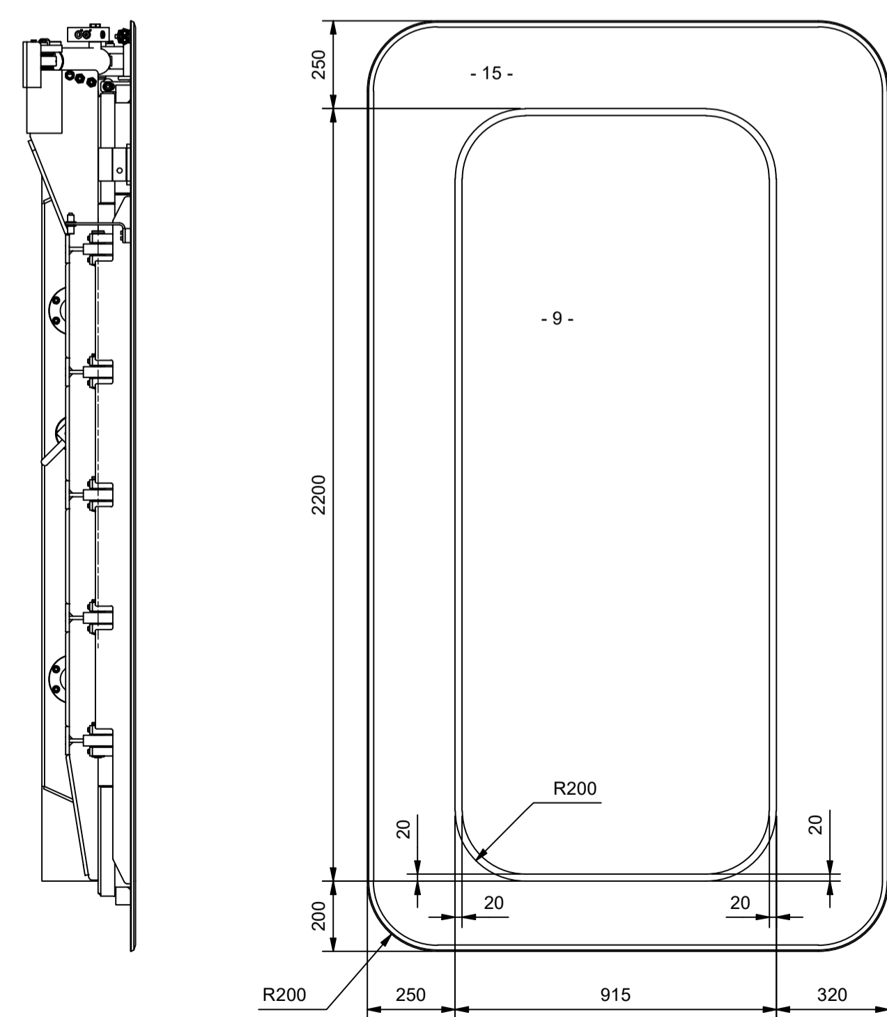
View from Outside Door (1 : 15)
