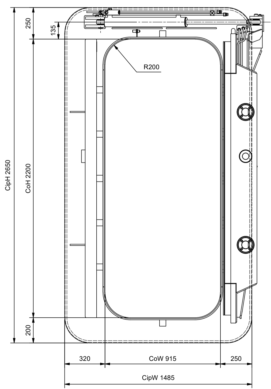
View from Inside Door (1 : 15) Opened and Unlocked
