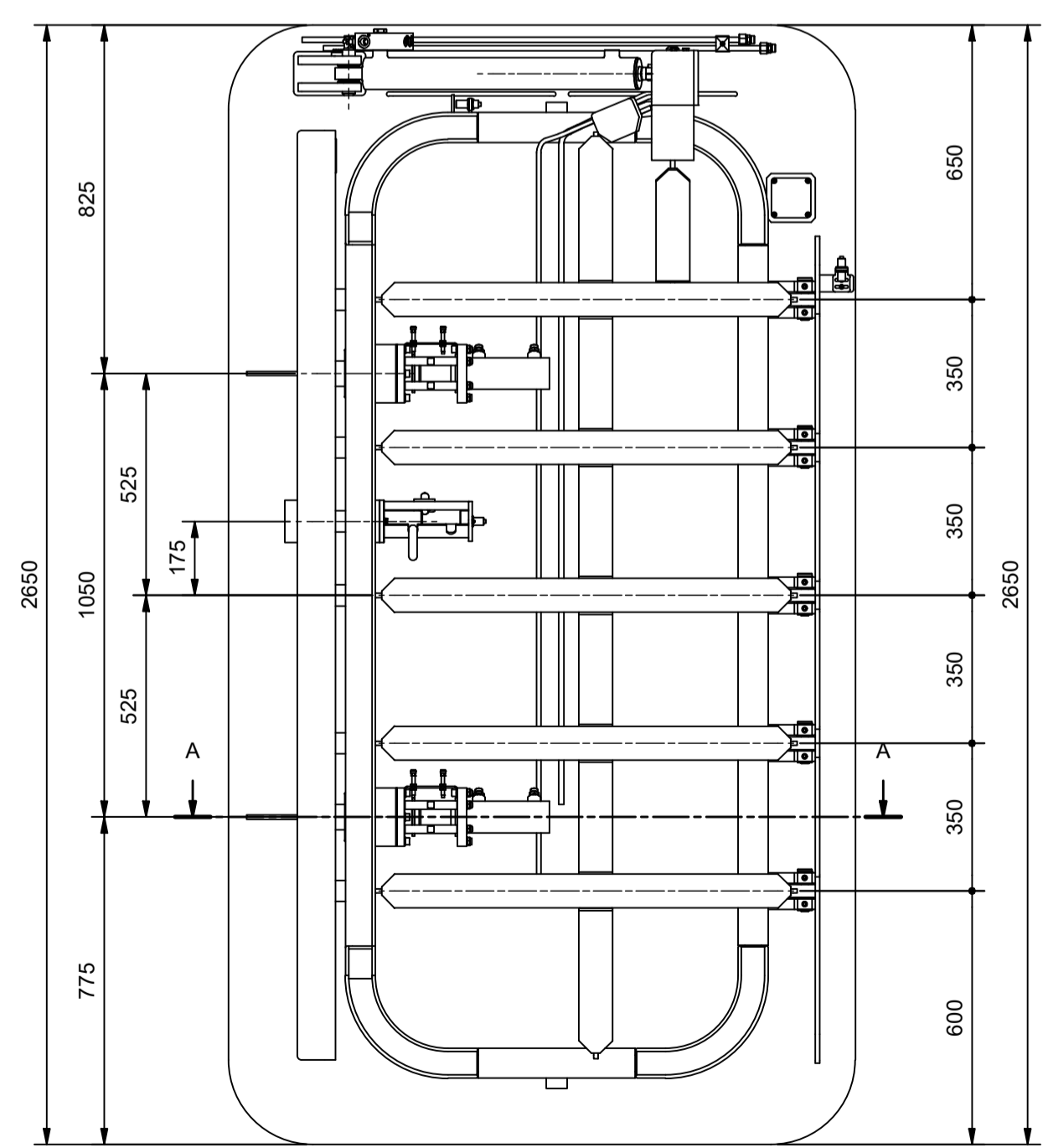
View from Inside Door (1 : 15) Closed and Locked
